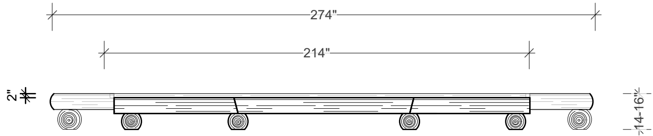
2 FRONT ELEVATION
